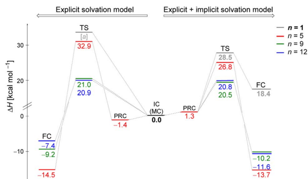
Fig. 2 Enthalpy change (in kcal mol -1 ) of the hydrolysis reaction of 1PrCl using the initial configurations of substrate–solvent clusters generated by Monte Carlo simulations. Left side displays the results obtained using exclusively explicit solvation model, and right side displays combined explicit + implicit solvation model results. Computed relative energies relative to their respective initial complexes, IC, at DFT-M06-2X/aug-cc-pVDZ level. TS refers to the transition state, PRC to pre-reactive complex, and FC to the final complex (products). [a] TS could not be optimized probably due to the necessity of stabilizing the charged leaving group, Cl - , by explicit solvent or a continuum medium.
