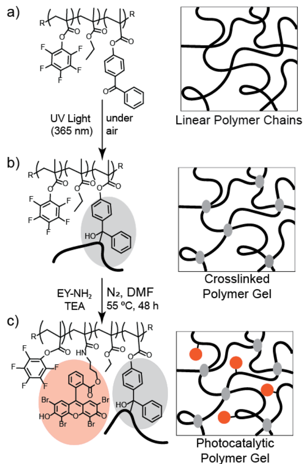
Fig. 1 (a) The chemical structure of the synthesized P(EtMA- co -BPMA- co -PFPPMA) copolymer. R groups represent the variety of chain ends produced from free radical polymerization. (b) The terpolymer was treated with UV light ( \lambda_{\text{max}} = 365 nm) to crosslink the polymer via C,H-insertion chemistry. (c) Treatment with a primary amine-bearing photocatalyst (Eosin Y; EY-NH 2 ) in presence of triethylamine (TEA) substituted the pentafluorophenyl moieties to yield the final photocatalytic cross-linked network.
