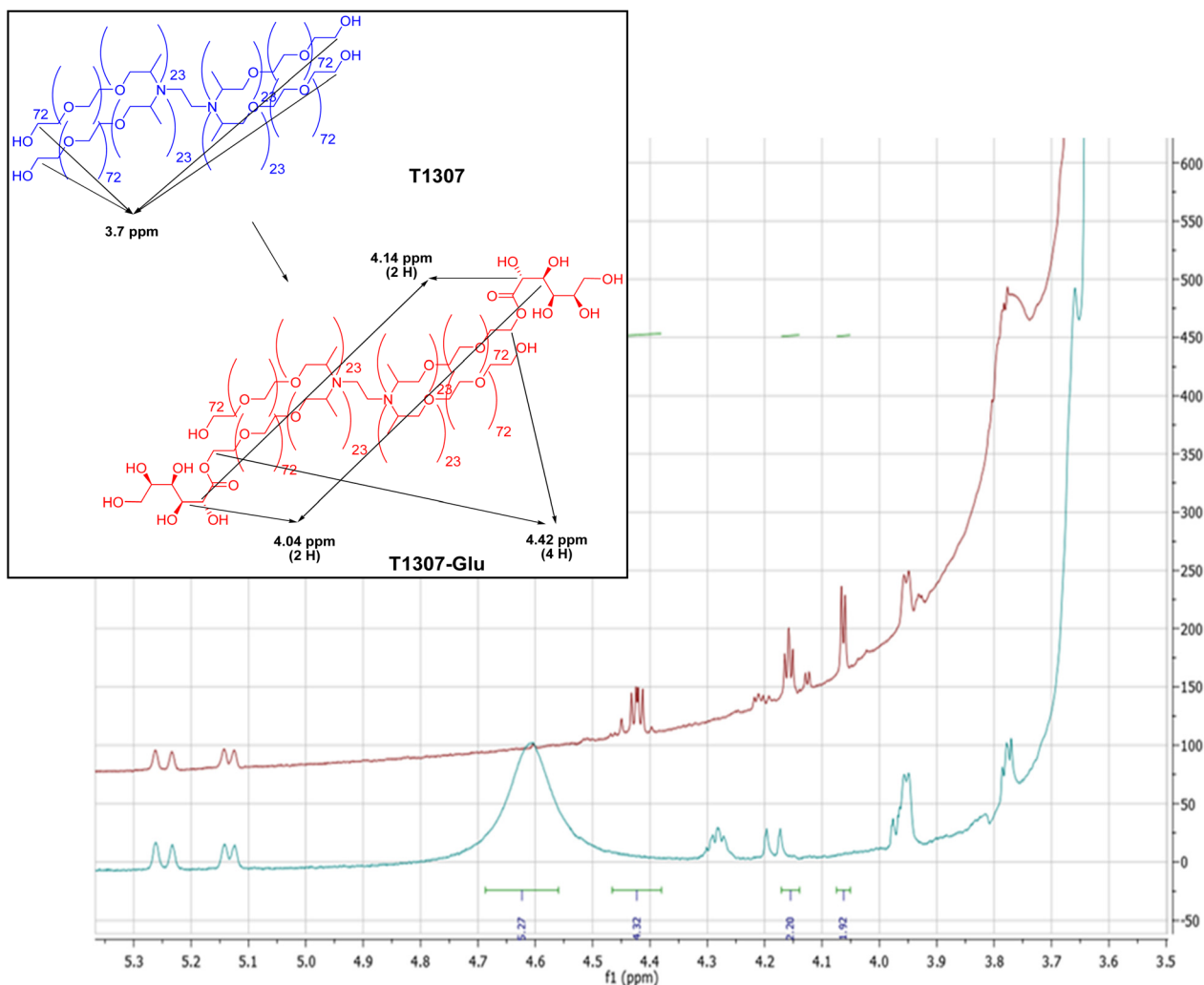
Fig. 2 Regions on the ^1\text{H} NMR spectra, between 3.5 and 5.3 ppm, corresponding to T1307-Glu (red) and T1307 (blue) copolymers (20% w/v, DMSO- d_6 , 298 K). Note: Except for the signal at 4.6 ppm, the integrations correspond to T1307-Glu.
