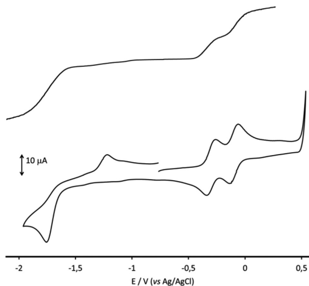
Fig. 4 Cyclic (bottom) and hydrodynamic (top) voltammetric responses recorded at a GC electrode in a \text{CH}_3\text{CN} solution of [\text{Rh}_{12}\text{In}(\text{CO})_{28}]^{3-} under CO atmosphere. [\text{N}^n\text{Bu}_4][\text{PF}_6] (0.1 mol dm −3 ) as the supporting electrolyte. Scan rate = 0.1 V s −1 .
