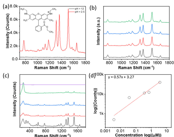
Fig. 6 (a) SERS response of PAA-grafted AgNPs for R6G at 0.36 μM. (b) SERS spectra of R6G PAA-grafted AgNPs at pH 2.5 for different solution spots. (c) SERS response of R6G in the concentration range of 3.6 nM–3.6 μM with PAA-grafted AgNPs. (d) Plotting the peak intensity at 1341 cm -1 against the concentration of R6G.
