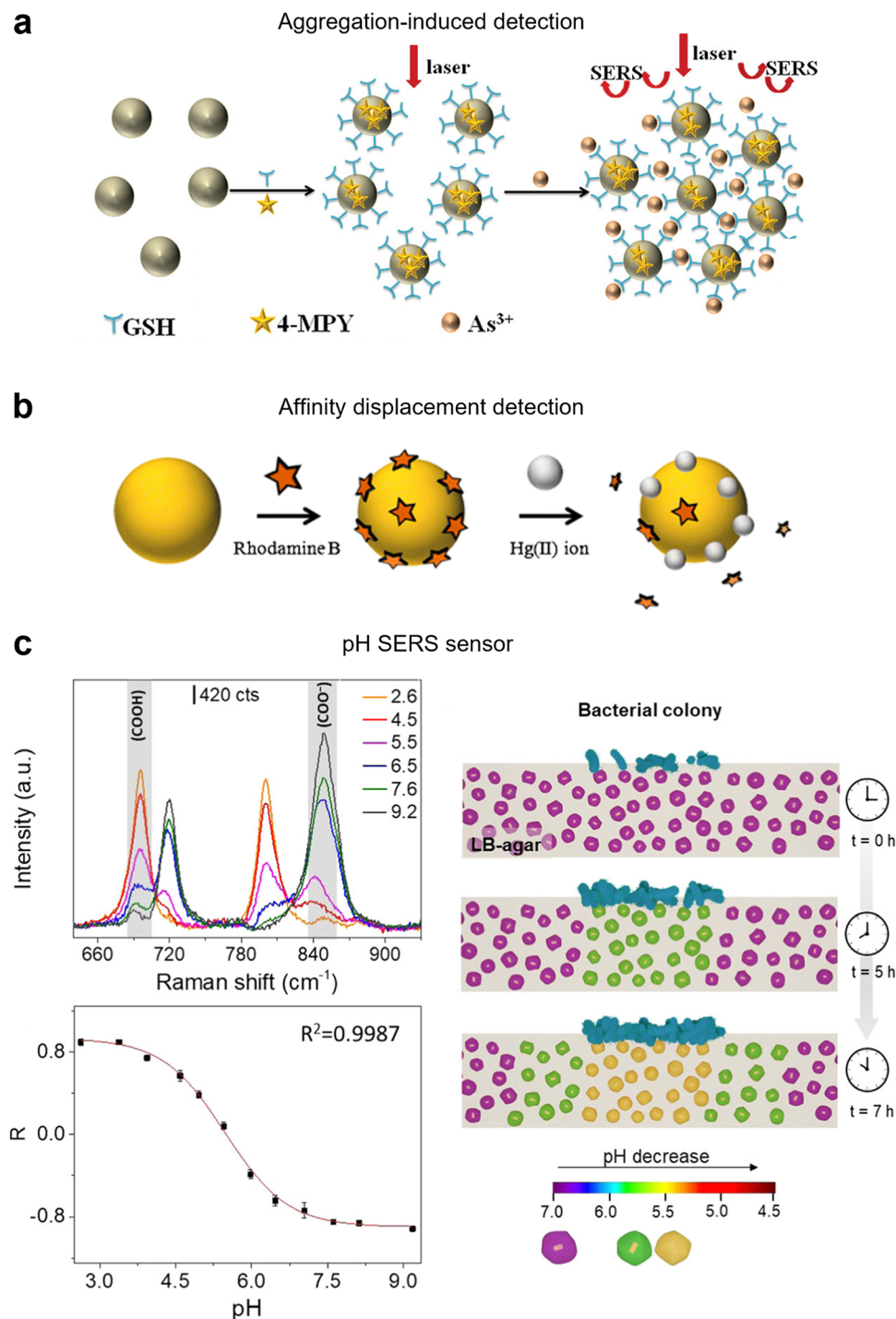
Fig. 9 Ionic SERS detection. (A) Schematic diagram of the detection of \text{As(III)} ion by the aggregation of nanoparticles in function of \text{As(III)} concentration. Reproduced from ref. 347 with permission from Elsevier Publication copyright 2020. (B) Schematic representation of the \text{Hg(II)} ion sensing mechanism based on the replacement of Rhodamine B molecules through the reduction of \text{Hg(II)} ions on the surface of gold nanoparticles. Reproduced from ref. 354 with permission from Springer publication, copyright 2009 (C) representative SERS spectra of 4-MBA at different pHs and experimental calibration curve or ratio R = (A_{695} - A_{848}) / (A_{695} + A_{848}) as a function of pH. Reproduced from ref. 355 with permission from ACS publication, copyright 2021.
