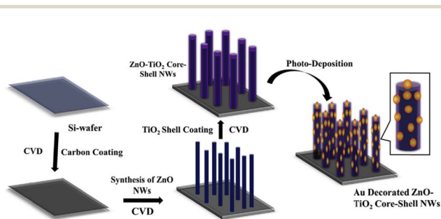
Fig. 10 Schematic representation of development of Au-NP decorated ZnO- \text{TiO}_2 core-shell NWs on the Si-wafer. Adapted with permission from ref. 102 Copyright (2018) American Chemical Society (ACS).
