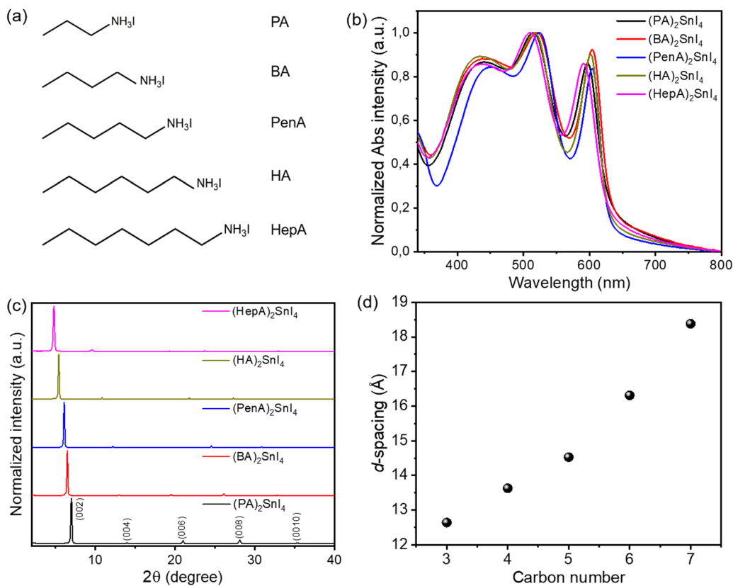
Fig. 1 (a) Chemical structures of PA, BA, PenA, HA, and HepA organic spacers. (b) UV-Vis absorption spectra and (c) XRD patterns of 2D tin halide perovskite films based on different organic cations. (d) Relationship between different cations (carbon numbers) and d -spacing values of (002) diffraction peaks.
