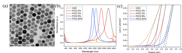
Fig. 26 (a) Transmission electron microscopy images of FICO 3% (diameter 20.2 \pm 1.8 nm). (b) Normalized absorption spectra of FICO NC samples with different doping levels. (c) Plots of (\alpha h\nu)^2 vs. photon energy ( h\nu ) for the FICO NC samples shown in (b). Reproduced from ref. 74 with permission from ACS, copyright 2019.
