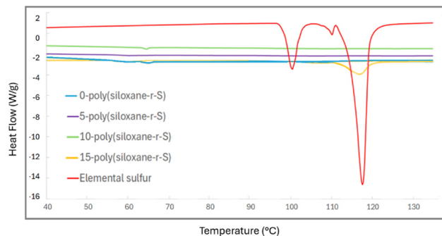
Fig. 9 Comparative DSC thermograms of X -poly(siloxane- r -S) ( X = wt% S); X = 0 (blue), 5 (purple), 10 (green), and 15 (yellow) and S_0 (red).
