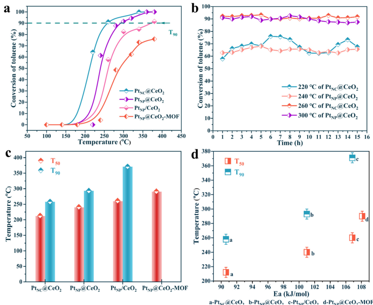
Fig. 1 The activity plot of \text{Pt}_{\text{NC}}@\text{CeO}_2 , \text{Pt}_{\text{NP}}@\text{CeO}_2 , \text{Pt}_{\text{NP}}/\text{CeO}_2 and \text{Pt}_{\text{NP}}@\text{CeO}_2\text{-MOF} catalysts (a), the stability tests of \text{Pt}_{\text{NC}}@\text{CeO}_2 and \text{Pt}_{\text{NP}}@\text{CeO}_2 under dry conditions (b), the comparison of T_{50} and T_{90} of each catalyst (c) and the catalytic activity versus E_a over the catalysts (d).
