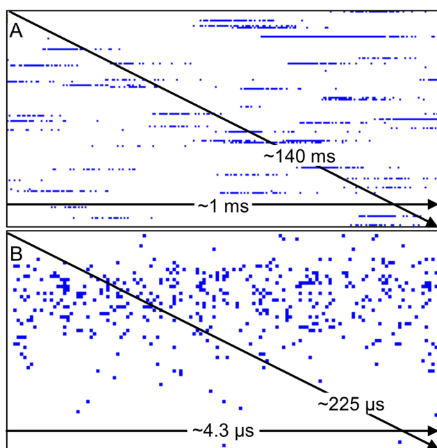
Fig. 2 Simplified visualization of spICP-MS data of a dispersion of 41 nm AuNP with nanosecond time resolution with a binary viewer program. (A) Several ion cloud signals during \sim 140 ms of acquisition. (B) Detector events in one individual ion cloud during \sim 225 \mu s data acquisition. Note: each blue logical pixel represents a byte with a value unequal to 0 (1 or more DE), each white logical pixel represents a byte with the value 0 (no DE).
