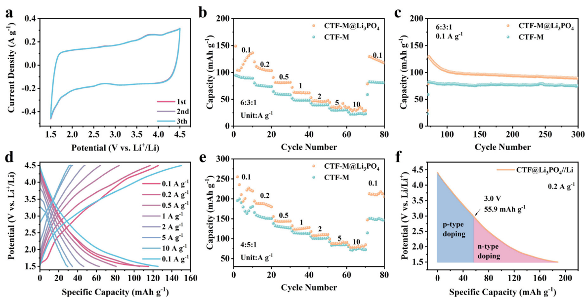
Fig. 3 (a) CV curves of CTF-M@Li 3 PO 4 /Li at 5 mV s -1 . (b) Rate performance of CTF-M and CTF-M@Li 3 PO 4 as the cathode with the CTF-M, ketjen black and PVDF weight ratio of 6 : 3 : 1. (c) Cycle performance of CTF-M and CTF-M@Li 3 PO 4 as the cathode with the CTF-M, ketjen black and PVDF weight ratio of 6 : 3 : 1 at 0.1 A g -1 . (d) Charge/discharge curves of CTF-M@Li 3 PO 4 /Li at various current densities. (e) Rate performance of CTF-M and CTF-M@Li 3 PO 4 as the cathode with the CTF-M, ketjen black and PVDF weight ratio of 4 : 5 : 1. (f) Discharge curve of CTF-M@Li 3 PO 4 /Li at 0.2 A g -1 , and its corresponding n-type and p-type doping capacity contributions.
