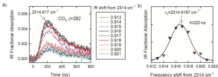
Fig. 3 (a) Transient signals of the CO 2 R(282) transition collected as a function of IR frequency. (b) The signals at t = 220 ns were fit to a Gaussian (black line) to identify the line-center frequency.
