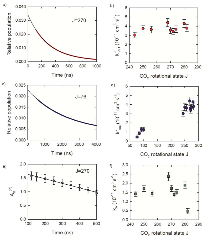
Fig. 9 (a) Population decay curve and fit for \text{CO}_2 J = 270 . (b) Relaxation rate constants for J = 244\text{--}282 . (c) Population decay curve and fit for \text{CO}_2 J = 76 . (d) Inclusion of relaxation rate constant for J = 76\text{--}100 . (e) Time-dependent alignment measurements for J = 270 and linear fit results. (f) Alignment decay constants for J = 244\text{--}282 .
