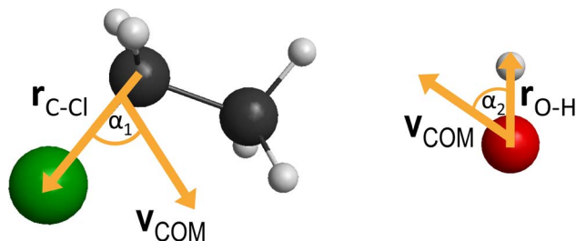
Fig. 1 The definitions of the initial attack angles: \alpha_1 is the angle between the C_{\alpha} -Cl bond vector and the center of mass velocity vector of the ethyl chloride while \alpha_2 is the angle between the O-H bond and the center of mass velocity vector of the hydroxide ion.
