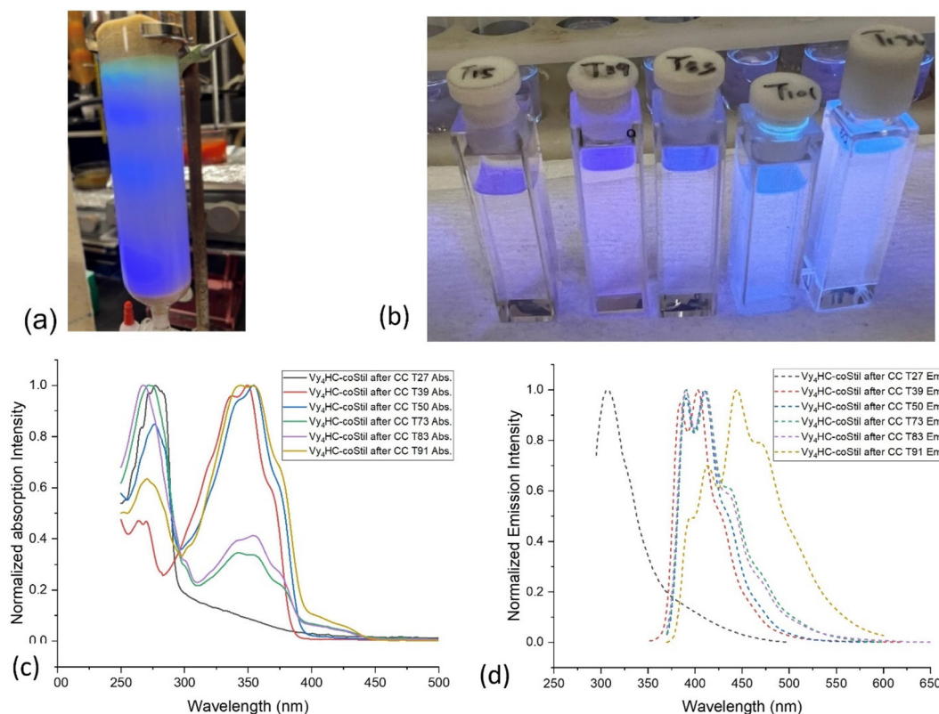
Fig. 2 (a) Optical images of Vy_4HC -coStil column illuminated with 365 nm light. Emission changes vs. vertical position on column. (b) Fluorescence emitted by selected fractions. Normalized (c) absorption (solid lines) and (d) emission (dashed lines) spectra of selected samples of the Vy_4HC coStil in DCM after column chromatographic separation.
