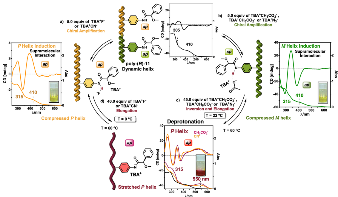
Fig. 23 (a) P and (b) M helix induction in poly-( R )- 11 by addition of 5.0 equiv. of TBA(A = fluoride or cyanide) or (A = acetate, benzoate or azide) respectively. Elongation and P helix induction in poly-( R )- 11 by addition of (c) 45.0 equiv. of TBA(A = acetate, benzoate or azide) at rt or (d) 40.0 equiv. of TBA(A = fluoride or cyanide) at 0 °C. Reproduced from ref. 189 with permission from Elsevier, copyright 2021.
