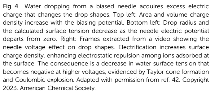
in electrospray, electrowetting, or electrospinning experiments. Fig. 4 shows that the excess charge in water lowers its surface tension and shape, thus affecting other surface properties. Viscosity and density are unaltered, showing that electrification does not affect bulk liquid.
