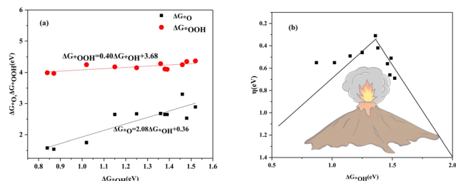
Fig. 13 (a) The scaling relationship of \Delta G_{\bullet\text{OOH}} and \Delta G_{\bullet\text{OH}} associated with \Delta G_{\bullet\text{O}} . (b) The volcano curve of the calculated \eta^{\text{ORR}} associated with \Delta G_{\bullet\text{OH}} .
