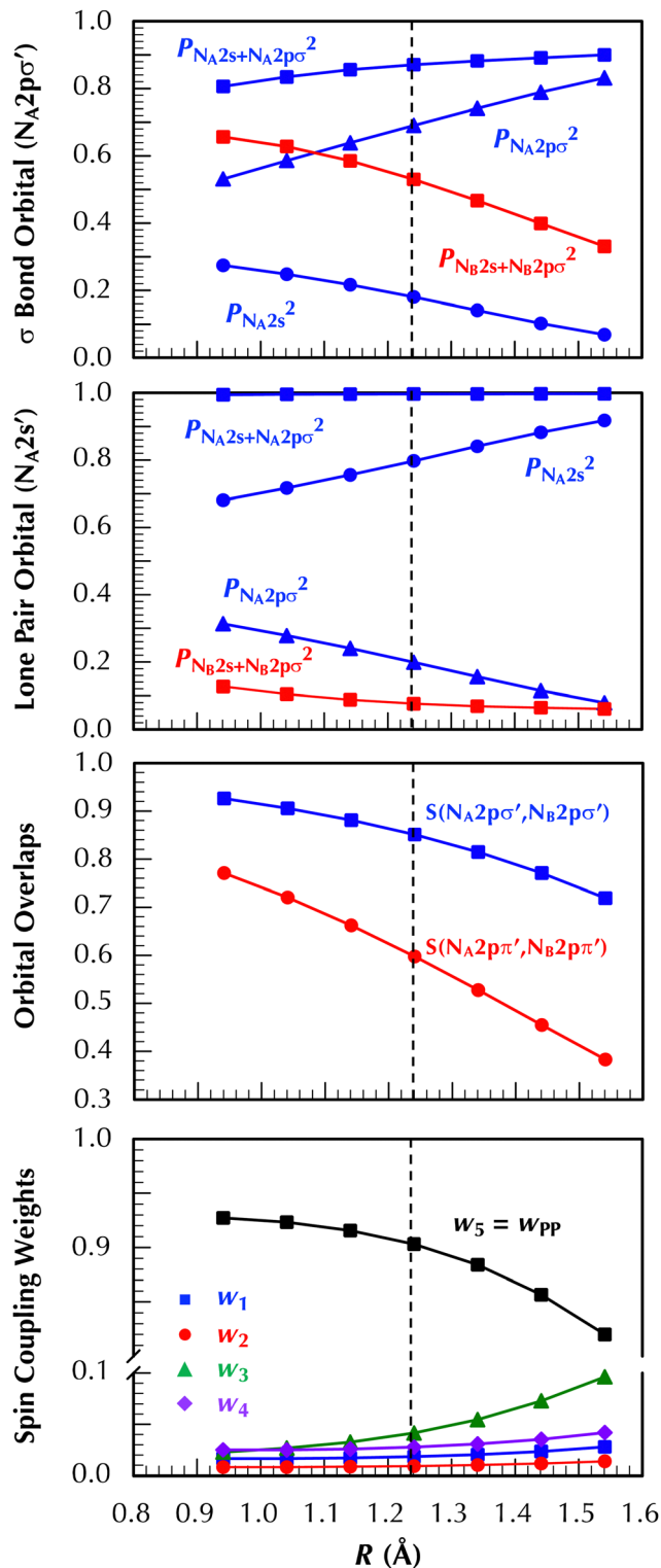
Fig. 8 Variation of selected characteristics of the SCGVb wavefunction in the vicinity of the minimum in \Delta E_{DEC}(R) for N_2 : atomic orbital analysis (top two plots), orbital overlaps (third plot) and spin-coupling weights (bottom plot). The dashed vertical line is drawn at the minimum ( R = 1.24 Å).
