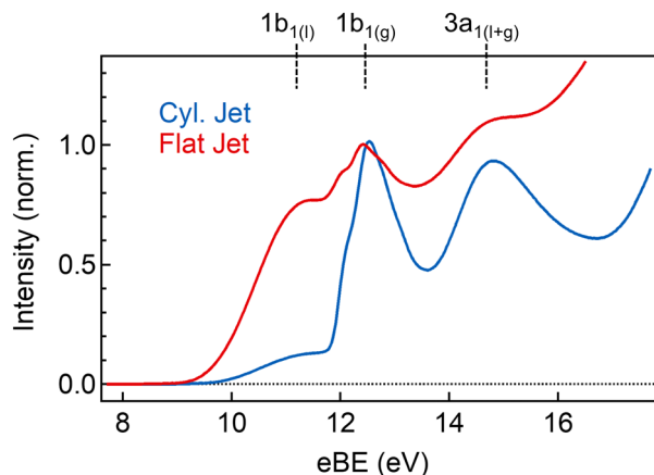
Fig. 3 One photon photoelectron spectra of an aqueous Ado solution depending on the mode of a jet; a 30- \mu m cylindrical jet (blue) and a flat jet (red).
