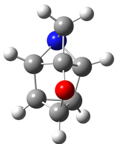
Fig. 3 A typical system in the GDB9-nonMR database in terms of size (H 7 C 7 NO) with 64 electrons.
