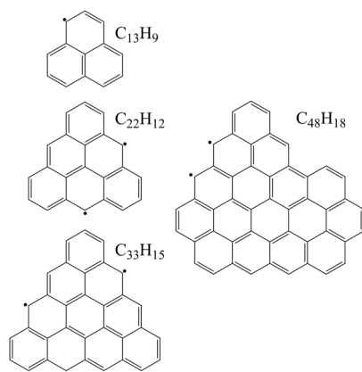
Fig. 9 PAH \pi -polyradicals. Left: Molecular structures of phenalenyl, \text{C}_{13}\text{H}_9 , and its triangular extensions, \text{C}_{22}\text{H}_{12} and \text{C}_{33}\text{H}_{15} , computed by the constrained optimization of the present study, eqn (5); right: the only \pi -biradical, \text{C}_{48}\text{H}_{18} , detected in the present kMC simulations.
