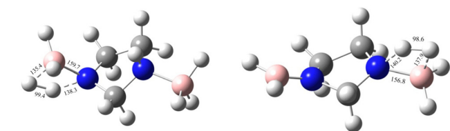
Fig. 8 The first and second transition-state structures with geometrical parameters for the uncatalysed dehydrogenation of IMBB at the CBS-QB3 level.
