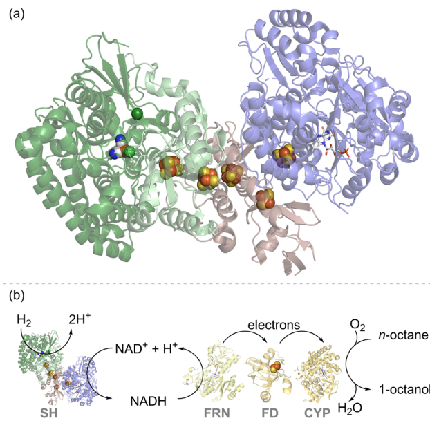
Fig. 2 (a) Structure of the soluble hydrogenase (SH) from Hydrogenophilus thermoluteolus showing the hydrogenase moiety in green, with the \text{NiFe(CO)(CN)}_2 catalytic site shown as spheres in elemental colours, and the \text{NAD}^+/\text{NADH} cycling moiety in blue, with the flavin catalytic site shown in stick form. Iron-sulfur electron relay clusters are shown in spheres in elemental colours. 21 (b) An engineered strain of Pseudomonas putida expressed SH and cytochrome P450 monooxygenase (CYP) together with the NADH-ferredoxin reductase (FRN) and ferredoxin (FD) needed for electron transfer. This enables enhanced activity for octane to octanol in the presence of \text{H}_2 , attributed to \text{H}_2 -driven \text{NAD}^+ reduction by the SH, as described in the ref. 22.
