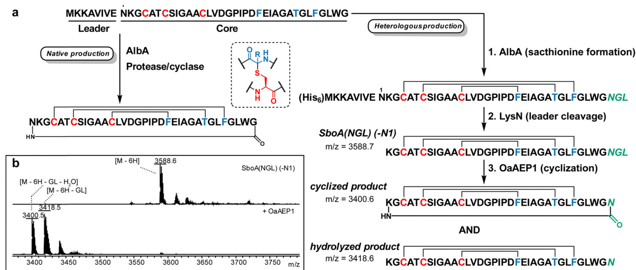
Fig. 2 (a) Production of subtilisin A from precursor peptide SboA. The structure of the sactionine linkage is shown in the dashed box. In the precursor peptide sequence, a His-tag and NGL motif for OaAEP1 cyclization was added. (b) MALDI-TOF MS result of (top) LysN-digestion of SboA(NGL) after co-expression with AlbA and (bottom) OaAEP1 cyclization of the purified product from the LysN digestion.
