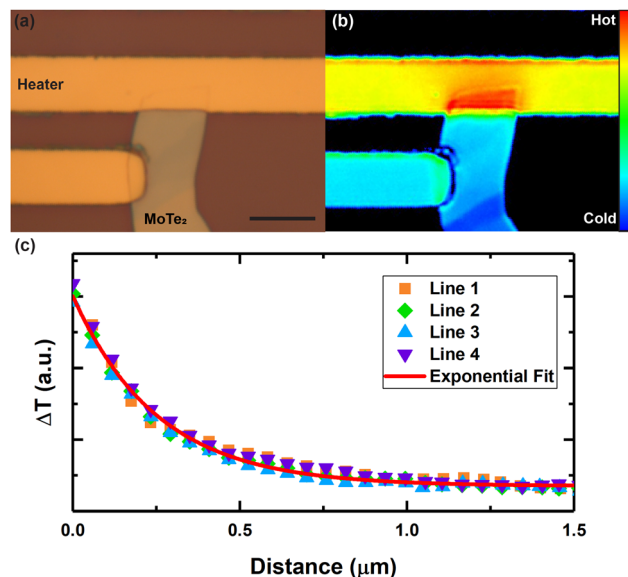
Fig. 4 (a) Optical image of the \text{MoTe}_2 device for thermal transport measurement. The scale bar is 5 \mu\text{m} . (b) Thermoreflectance map of the sample surface with 5 \text{ V} supplied to the heater. Temperature decay curves were taken along the sample perpendicular to the heater. (c) Temperature decay curves and their corresponding exponential fit for thermal conductivity extraction.
