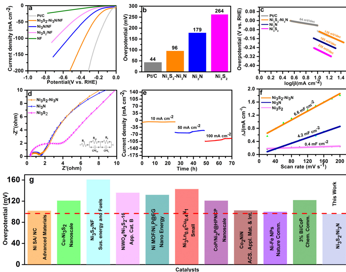
Fig. 5 (a) The polarization curves of all the catalyst for the HER. (b) Overpotential values of the catalysts at 10 mA cm -2 of current density. (c) The Tafel plots showing the Tafel slope values of all the catalysts. (d) The Nyquist plots for the determination of R_{ct} using an equivalent circuit shown in the inset image. (e) Stability study using chronoamperometry. (f) Double layer capacitance values of Ni 3 S 2 -Ni 3 N, Ni 3 S 2 and Ni 3 N. (g) Comparison of our catalyst with the recently reported catalysts for the HER.
