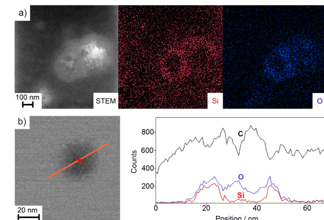
Fig. 3 Structure of FR/CC@SiO 2 core-shell nanoparticles: (a) EDXS area scans with element mapping and (b) EDXS line scan with concentration profile at the position of the orange line on the STEM image.
