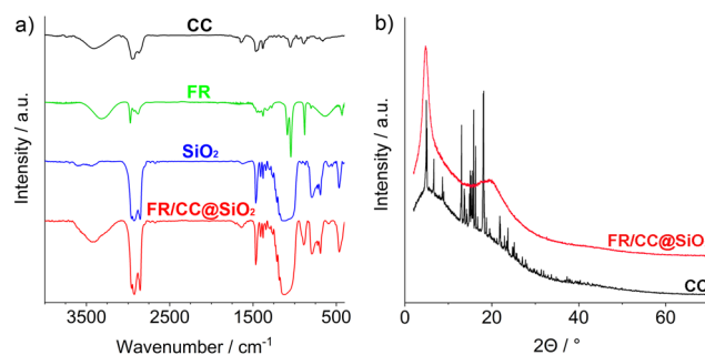
Fig. 4 Chemical composition of the as-prepared FR/CC@SiO 2 core-shell nanoparticles: (a) FT-IR spectra with FR, CC, and SiO 2 as a reference (SiO 2 prepared by hydrolysis of OTES); (b) XRD patterns with CC as a reference.
