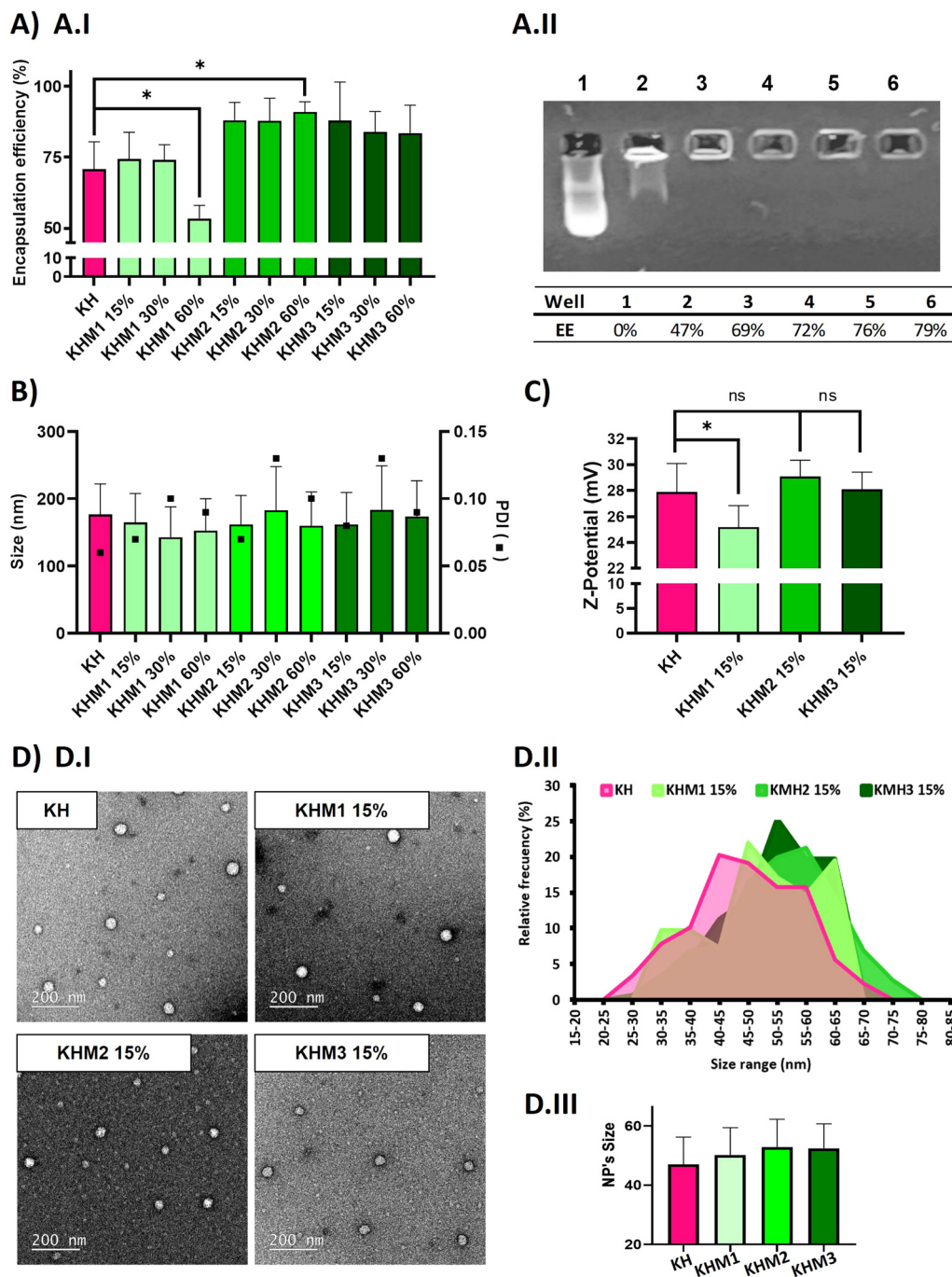
Fig. 2 Physico-chemical analysis of different nanoparticle formulations containing \alpha -mannose. In pink, the control KH, in soft green the formulations containing Man1-CK3, in medium green the formulations containing Man2-CK3 and in dark green the ones containing Man3-CK3. Polyplexes were prepared using mRNA eGFP with polymer at 25 : 1 ratio (w : w), diluted with RNase-free water. Results are shown as mean and standard deviation of triplicates. (A) Average encapsulation efficiency of the different tested formulations with (A.I) Ribogreen ® and (A.II) Gel retardation assay (quantified by ImageJ) of Man1-CK3 formulations, using DNA as the genetic material. (1-Free pDNA 2-KHM1 60% 3-KHM1 45% 4-KHM1 30% 5-KHM1 15% 6-KH) (B) size (bars) and Polydispersity Index (PDI) (square) of the analyzed populations by DLS. (C) Z-potential by DLS. p -Value: 0.05 (*), 0.01 (**), < 0.001 (***) (D and D.I) TEM images of NP formulations KH, KHM1 15%, KHM2 15 and KHM3 15% with 12000X amplifications. (D.II) Analysis of the nanoparticles size distribution by ImageJ. (D.III) Mean and standard deviation of the nanoparticles.
