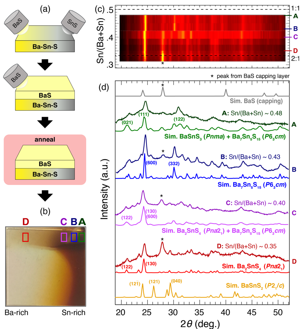
Fig. 3 (a) A schematic of the three-step anneal plus capping layer process for combinatorial Ba–Sn–S thin films. (b) A photograph of a representative sample with the regions of interest boxed. (c) A heatmap of XRD patterns in the top row of the annealed sample. (d) Representative experimental XRD patterns for the four regions (A–D) marked with rectangles in (b), with simulated ("Sim.") patterns and indices from crystal structures in the ICSD using a pymatgen Scherrer peak-broadening algorithm.
