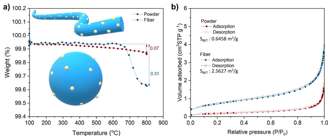
Fig. 4 Exsolution process of LCNT perovskite materials under chemical reduction. (a) Weight loss of LCNT samples reduced in 5% H 2 /N 2 from 100 to 800 °C, (b) N 2 adsorption–desorption isotherms and BET surface area of samples.
