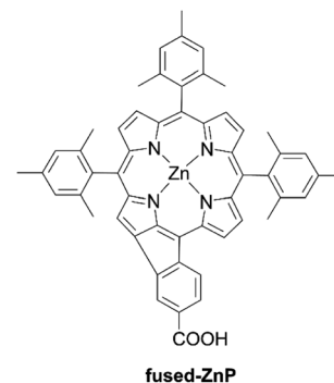
Fig. 10 Chemical structure of fused-ZnP.
