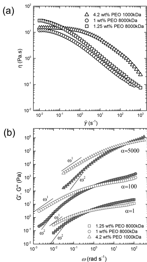
Fig. 4 (a) Flow sweep experiments showing the variation of bulk viscosity \eta_0 with shear rate \dot{\gamma} and (b) frequency sweep experiments for different polymer solutions carried out at a strain of 1%. Closed symbols and open symbols represent storage ( G'(\omega) ) and loss moduli ( G''(\omega) ) respectively.
