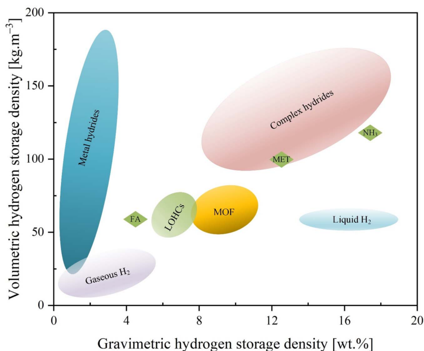
Fig. 2 Volumetric and gravimetric densities (based on storage materials and storage vessels) of different hydrogen storage technologies; circular carriers: ammonia (NH 3 ), methanol (MET), and formic acid (FA). 48
