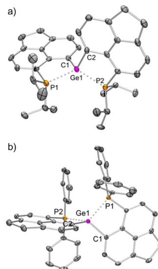
Fig. 3 Molecular structures of (a) \mathbf{3}^{\text{Pr}} and (b) \mathbf{3}^{\text{Ph}} (H atoms, solvent molecules and triflate anions have been removed for clarity; thermal ellipsoid 50%). Selected bond lengths [Å] and angles [ ^\circ ]: (a) Ge1–C1 = 1.923(5) , Ge1–C2 = 1.923(5) , Ge1–P1 = 2.350(1) , Ge1–P2 = 2.363(1) ; C1–Ge1–C2 = 112.5(2) , P1–Ge1–P2 = 122.4(1) , C1–Ge1–P1 = 90.9(2) , C2–Ge1–P2 = 91.4(2) , C1–Ge1–P2 = 120.8(2) , C2–Ge1–P1 = 121.2(2) ; (b) Ge1–C1 = 1.924(3) , Ge1–C2 = 1.920(3) , P1–Ge1 = 2.344(1) , Ge1–P2 = 2.338(1) ; C2–Ge1–C1 = 126.8(1) , C2–Ge1–P2 = 91.5(1) , C1–Ge1–P2 = 116.1(1) , C2–Ge1–P1 = 115.7(1) , C1–Ge1–P1 = 91.2(1) , P2–Ge1–P1 = 118.1(1) .
