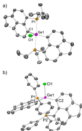
Fig. 2 (a) Molecular structures of (a) \mathbf{2}^{\text{Pr}} and (b) \mathbf{2}^{\text{Ph}} (H atoms, solvent molecule and triflate anion have been removed for clarity; thermal ellipsoid 50%). Selected bond lengths [Å] and angles [ ^\circ ]: (a) Ge1–Cl1 = 2.228(2) , Ge1–C1 = 1.988(4) , Ge1–P1 = 2.643(1) ; C1–Ge1–C1 = 147.9(2) , Cl1–Ge1–C1 = 106.1(1) , Cl1–Ge1–P1 = 86.9(1) , P1–Ge1–P1 = 173.9(1) ; (b) Ge1–C1 = 1.922(3) , Ge1–C2 = 1.926(3) , Ge1–Cl1 = 2.215(1) , Ge1–P1 = 2.357(1) ; C1–Ge1–C2 = 120.0(1) , C1–Ge1–Cl1 = 104.8(1) , C2–Ge1–Cl1 = 104.2(1) , C1–Ge1–P1 = 91.1(1) , C2–Ge1–P1 = 135.5(1) , Cl1–Ge1–P1 = 96.4(1) .
