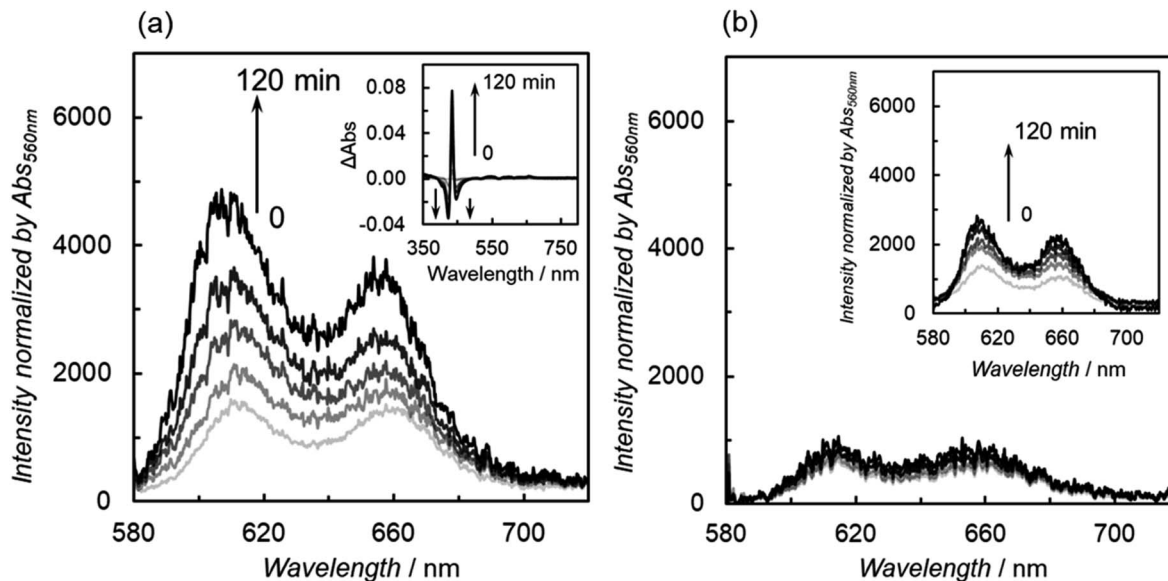
Fig. 8 (a) Fluorescence spectral changes (0–120 min) of the \text{CO}_2 -saturated DMA containing \text{ZnP-6Bpy=Re}^{\text{Br}} ( 3 \mu\text{M} ) in the presence of 50 \mu\text{M} of BIH during irradiation at 560 \text{ nm} . Inset shows differential UV-vis absorption spectra during the irradiation. (b) Fluorescence spectral changes (0–120 min) of the \text{CO}_2 -saturated DMA-TEOA (4 : 1 v/v) containing \text{ZnP-6Bpy=Re}^{\text{Br}} ( 3 \mu\text{M} ) in the presence of 50 \mu\text{M} of BIH during irradiation at 560 \text{ nm} . Inset shows fluorescence spectral change in the presence of 6.7 \text{ mM} phenol.
