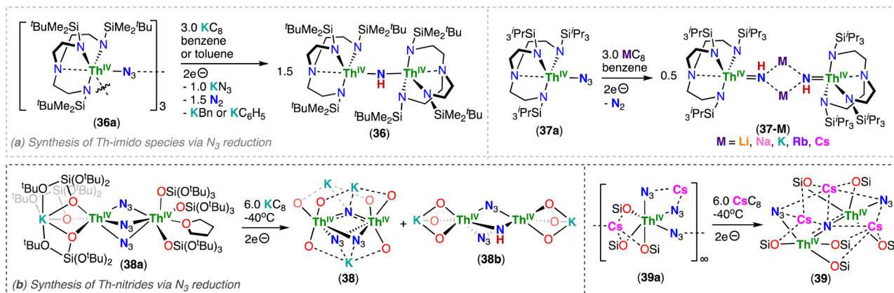
Scheme 8 Synthesis of thorium (a) imidos and (b) nitrides supported by triamidoamine ( \text{TREN}^{\text{DMBS}} and \text{TREN}^{\text{TIPS}} ) and siloxide ( -\text{OSi}(\text{O}^t\text{Bu})_3 ) ligands, respectively.
