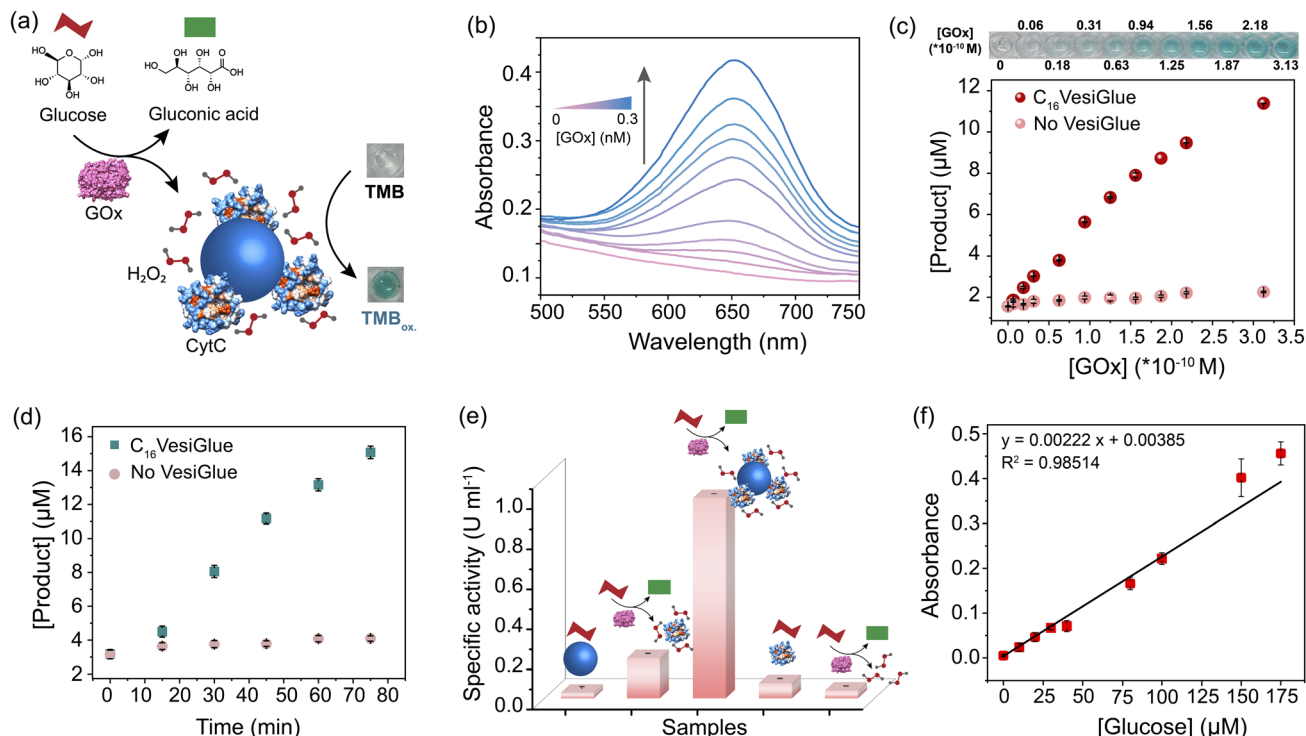
Fig. 5 Cascade reaction in the Vesiglu system. (a) Schematic of a biocatalytic cascade where glucose is oxidized by glucose oxidase (GOx), producing \text{H}_2\text{O}_2 that serves as the substrate of CytC glued onto Vesiglu. (b) UV-vis traces of oxidized TMB ( \text{TMB}_{\text{ox}} ) with increasing GOx concentration, in the catalytic cascade. (c) \text{C}_{16}\text{Vesiglu} mediated oxidation of the substrate by the biocatalytic cascade. The concentration of \text{TMB}_{\text{ox}} is measured through the absorbance at \lambda_{\text{max}} 650 nm. Varying concentrations of GOx (0–0.3 nM) in the presence (red) and absence (peach) of \text{C}_{16}\text{Vesiglu} show the linear dependency on the enzyme concentration. The digital photos above the graph show the color of the \text{TMB}_{\text{ox}} in presence of \text{C}_{16}\text{Vesiglu} . (d) Rate of product formation ( \text{TMB}_{\text{ox}} ) in the presence (green) and absence (peach) of Vesiglu demonstrating the effect of CytC anchoring on the cascade reaction. (e) Specific activity of CytC under different conditions verifying the role of a complete system in catalyzing the cascade reactions. The shapes of (a) are used that have the same meaning. (f) The GOx/CytC/ \text{C}_{16}\text{Vesiglu} cascade reaction with increasing glucose concentration (0–175 \mu\text{M} ). The black solid line represents a linear fit of the data. n = 3 technical replicates, mean \pm SD for all the studies.
