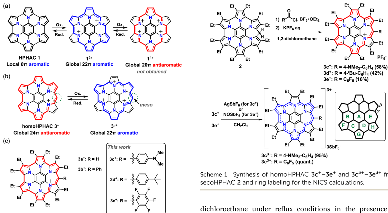
Fig. 1 (a) Chemical structures of HPHAC 1 and its cationic species. (b) Resonance structures of antiaromatic homoHPHAC 3 ^+ and aromatic 3 ^{3+} . (c) HomoHPHAC 3a ^+ –3e ^+ with the various substituents studied in this work.
