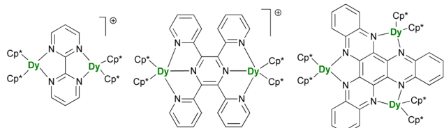
Fig. 9 Molecular structures of \{[(\text{Cp}^*)_2\text{Dy}](\mu\text{-bipym})\}^+ , 196 \{[(\text{Cp}^*)_2\text{Dy}](\mu\text{-tppz})\}^+ , 197 and (\text{Cp}^*)_6\text{Dy}_3(\mu_3\text{-HAN}) . 198
