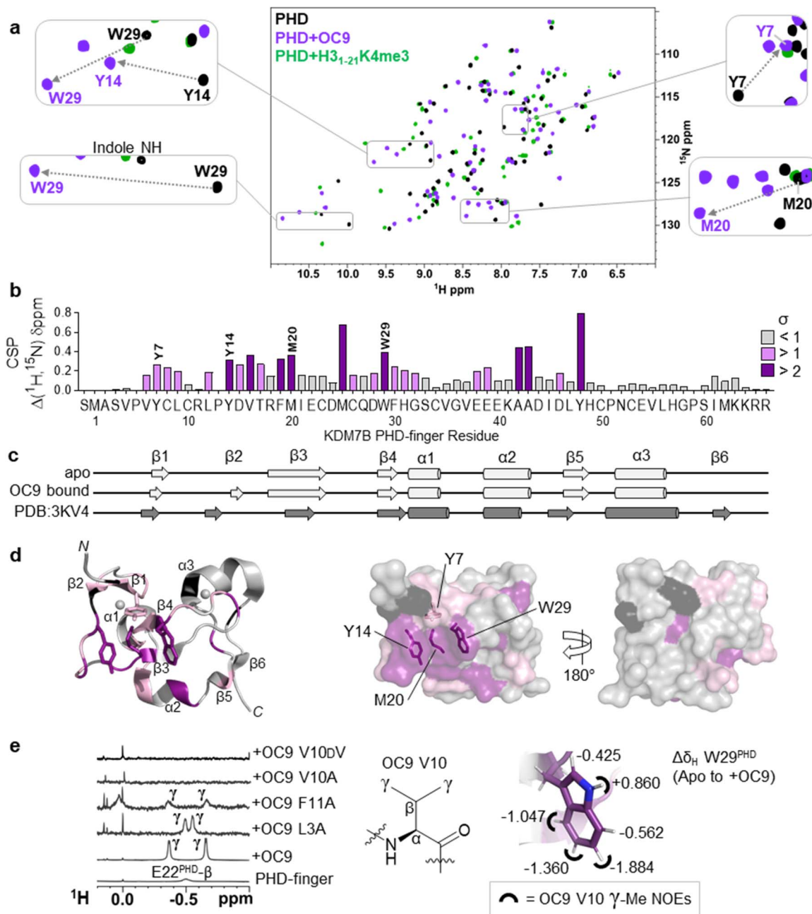
Fig. 4 Protein NMR reveals valine contacting of the aromatic cage. (a) ^1\text{H} - ^{15}\text{N} HSQC of KDM7B PHD-finger in the apo (black) or bound forms with OC9 (purple, 1 : 1) or H _3 K _4 me _3 (green, 3 : 1). (b) ^1\text{H} and ^{15}\text{N} chemical shift changes for apo vs. + OC9 were combined and weighted to give chemical shift perturbation (CSP) ( \Delta\delta ) values. Standard deviation ( \sigma ) of \Delta\delta are indicated ( >1 pink, >2 purple). (c) TALOS+ predicts similar secondary structure elements in apo and OC9-bound solution protein complexes (light grey) to those found in PDB ID 3KV4 (dark grey). (d) Mapping of CSP \sigma from (b) onto PDB ID 3KV4 shows OC9 binding surfaces primarily along one face, which presents the cage (annotated residues). (e) Shielded ^1\text{H} -NMR signals centered around -0.5 ppm belonging to the OC9 V10 \gamma -methyl groups are observed in some OC9-PHD complexes, but not in apo protein, or complexes with OC9 V10A and OC9 V10D _V . The V10 ^{\text{OC9}} \gamma -methyl signals have NOE interactions (black semi-circles) with the W29 ^{\text{PHD}} indole, which itself is shielded upon binding of OC9 (indicated by \Delta\delta_{\text{H}} values).
