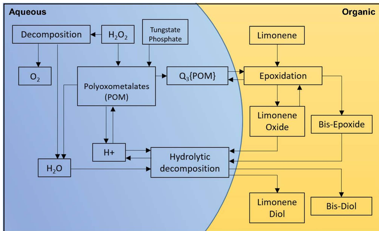
Fig. 5 Overall reaction scheme for the epoxidation of (R)-(+)-limonene, the formation of oxidative species, the decomposition of H 2 O 2 and the hydrolytic decomposition of the epoxides. Each reaction is visualized in the schematic diagram (an aqueous phase is shown in blue, while an organic phase is shown in gold).
