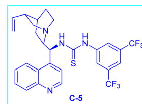
Scheme 10 Organocatalytic asymmetric [3+2] cycloaddition for the assembly of \text{CF}_3 -embedded spirooxindoles 22 .
