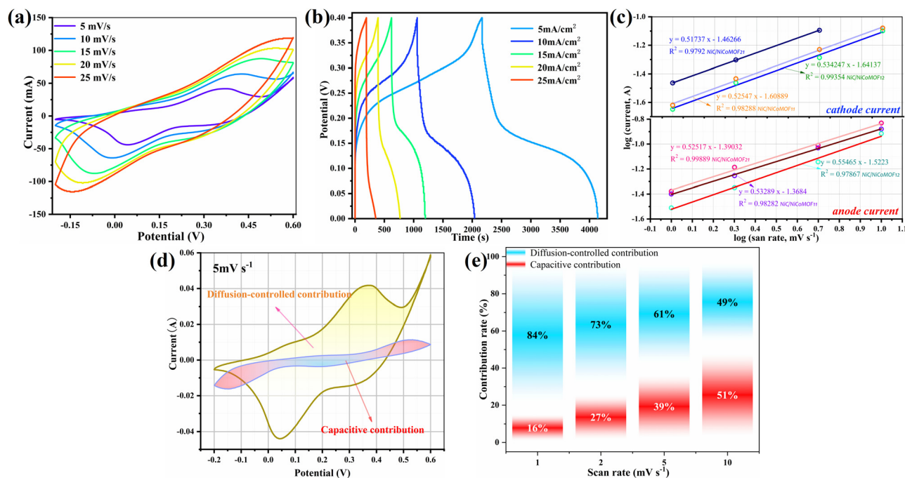
Fig. 6 CV curves of NiC/NiCoMOF21 at 5–25 mV s -1 . (b) GCD curves of NiC/NiCoMOF21 at 5–25 mA cm -2 . (c) Linear plot between log( i ) and log( v ) at different potentials. (d) The capacitive and diffusion-controlled contributions in the electrode process.
