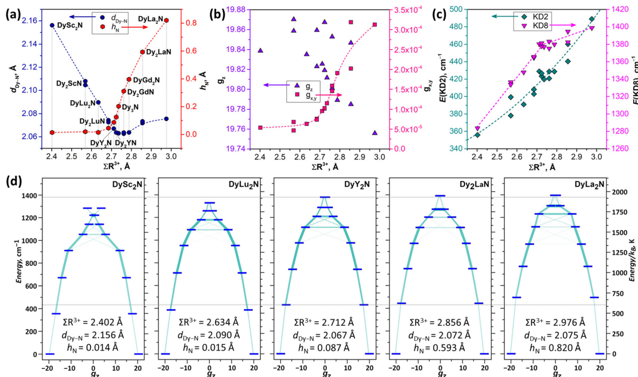
Fig. 5 (a) Dy–N bond lengths ( d_{\text{Dy-N}} ) and M 3 N pyramid height (elevation of N above the plane of metal atoms, h_{\text{N}} ) in DFT-optimized DyM 2 N@C 80 and Dy 2 MN@C 80 molecules (M = Sc, Lu, Y, La, Gd) plotted versus the sum of Shannon's ionic radii of metals in the M 3 N cluster ( \Sigma R^{3+} ). (b) Components of the pseudospin g -tensor, g_z and g_{xy} (root mean square of g_x and g_y ) for the Dy 3+ ground state Kramers doublet (KD1) in the same set of molecules. (c) The energy of the first excited KD (KD2) and the total ligand-field splitting (KD8) in the same set of molecules. Dashed lines in (a) and (b) are a spline interpolation added to guide the eye; in (c), the dashed line for E(\text{KD2}) is a quadratic fit. (d) Dy 3+ ligand-field splitting with transition probabilities in selected M 3 N@C 80 molecules along with their \Sigma R^{3+} , d_{\text{Dy-N}} , and h_{\text{N}} parameters; dotted lines are guides to the eye and mark the KD2 and KD8 energies in Dy 2 N@C 80 . Ligand-field splitting and pseudospin g -tensor parameters used in (b–d) are computed ab initio at the CASSCF/RASSI-SO level using DFT-optimized molecular structures.
