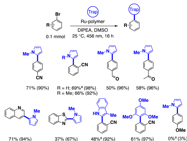
Fig. 6 The C–H arylation products obtained from (hetero)aryl bromides and heterocycles. Yields are determined by ^1\text{H} NMR spectroscopy using 1,3,5-trioxane as an internal standard. Parentheses indicate the percent conversion of the aryl bromide. a Reaction time was 32 hours.
