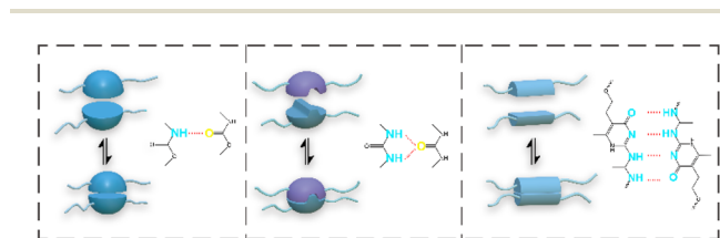
Fig. 2 The three typical hydrogen bonds in PU.
