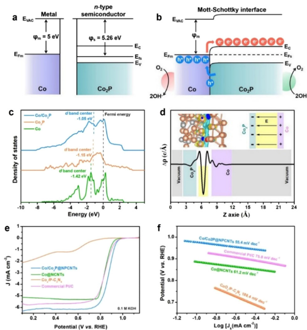
Fig. 8 Energy band diagrams for Co metal and n-type Co 2 P semiconductor (a) before and (b) after Schottky contact. (c) Density of states (DOS) for Co/Co 2 P, Co and Co 2 P models. (d) Charge density difference for the Co/Co 2 P heterojunction. (e) ORR polarization curves and (f) Tafel plots of different electrocatalysts. (a)–(c) Reproduced with permission from ref. 82, 2021, Elsevier.
