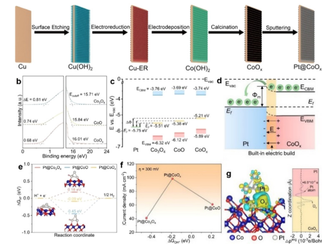
Fig. 4 (a) A schematic illustration of the synthesis of Pt@CoO x . (b) UPS spectra and (c) the energy-band alignment diagram of CoO, CoO x , and Co 3 O 4 with respect to Pt. (d) A schematic illustration of the Schottky junction. (e) Adsorption free energies of H* on Pt@CoO x and some referenced samples. (f) Adsorption free energies of OH* on Pt@CoO x and some referenced samples. (g) Iosurfaces of charge density difference (left) and planar-average charge density plot (right) of Pt@CoO x . Reproduced with permission from ref. 41, 2022, Wiley-VCH.
