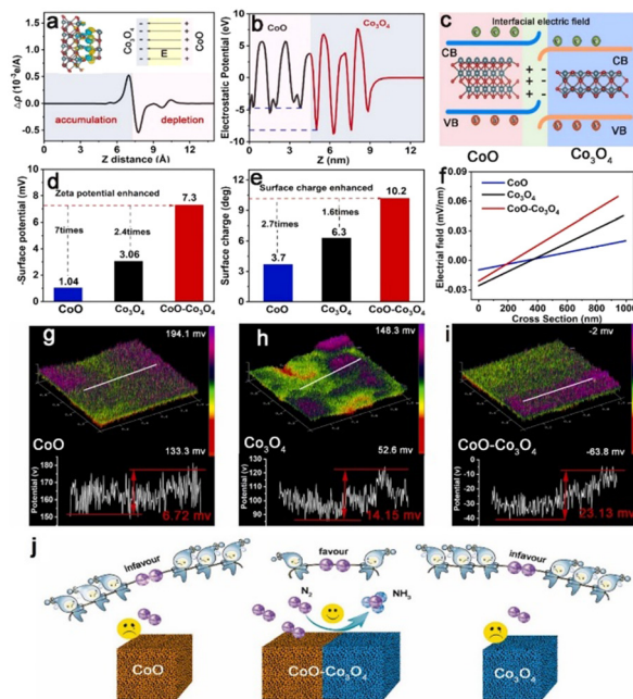
Fig. 9 (a) Charge density difference and (b) electrostatic potential profile for CoO–Co 3 O 4 . (c) A schematic of the interface charge transfer process in the CoO–Co 3 O 4 heterostructure. (d) The Zeta potentials, (e) surface charge, and (f) intense distributions of electric field of CoO, Co 3 O 4 and CoO–Co 3 O 4 . (g)–(i) The 3D surface potential distribution and corresponding line scanning surface potential profile of CoO, Co 3 O 4 and CoO–Co 3 O 4 . (j) A schematic diagram presenting the interfacial electric field engineered in CoO–Co 3 O 4 heterostructure for boosting electrocatalytic NRR. Reproduced with permission from ref. 26, 2023, Elsevier.
