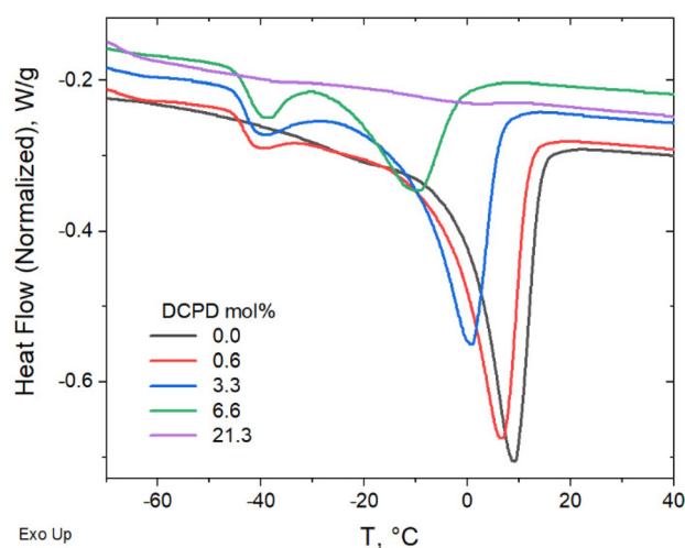
Fig. 8 Fusion of enthalpy comparison after 1 hour annealing at -50^\circ\text{C} to allow full crystallization.
